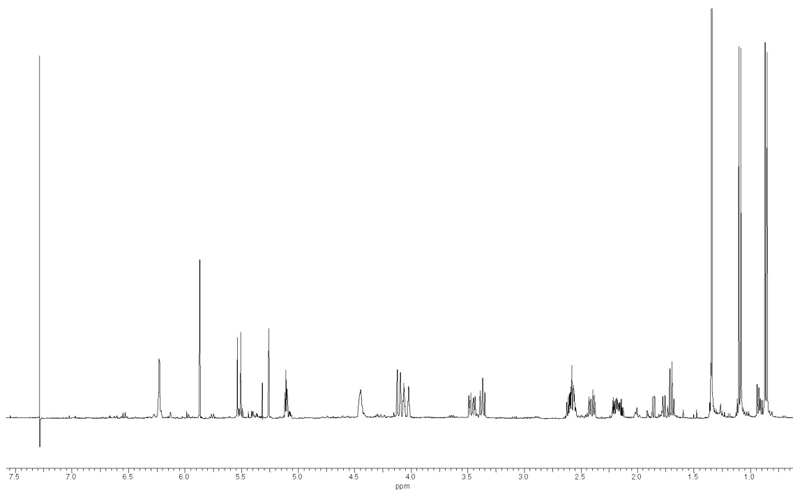
Figure 5S. ^1\text{H} NMR spectrum of 4
