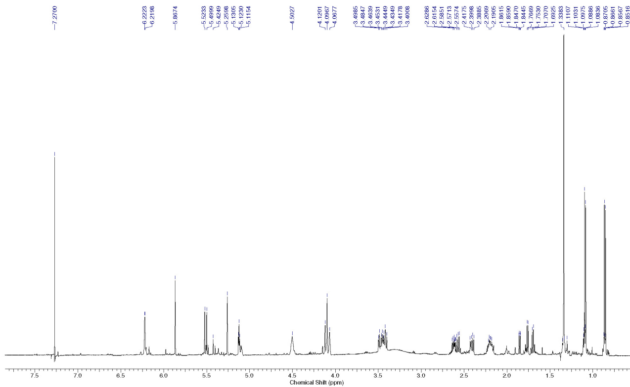
Figure 4S. ^1\text{H} NMR spectrum of 3
